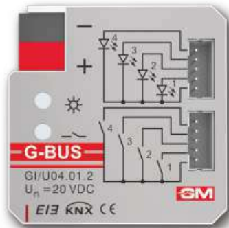
Universal Interface 4 - Fold GI/U04.01.2 Dimension: 45.5x45.5x12 mm
