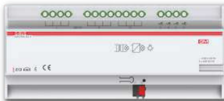
Dimmer Actuator 4 - Fold GA/D04.03.2 500W Incandendent load Dimension: 216x91x64 mm
